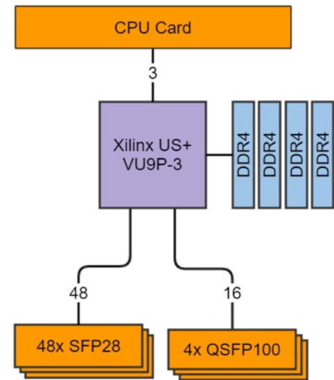
Arista 7132LB-48Y4C System Architecture
