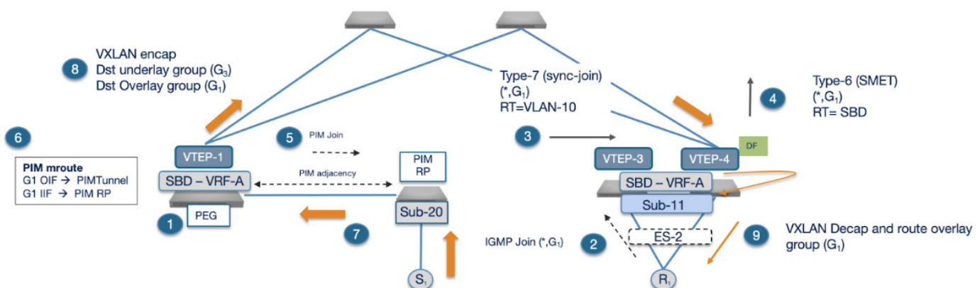
Figure 8: EVPN layer 3 multicast routing forwarding model with OISM and external PIM domain
